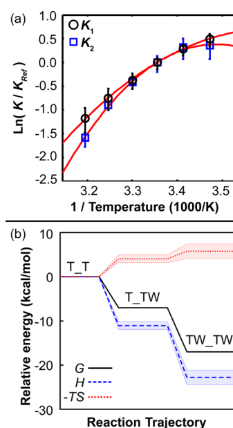
Figure 5. Extended van't Hoff analysis reveals a stepwise increase in bondedness and order of the Trp–TRAP–solvent system upon Trp binding. (a) The van't Hoff plot illustrates curvature for both steps, which are each fit with slope \Delta H and curvature \Delta C_p . Error bars are 95% confidence intervals from a Monte Carlo error analysis propagated from the original stopped-flow time courses. (b) Energetic contributions from enthalpy H and entropy -TS at 25\text{ }^{\circ}\text{C} along the reaction coordinate reveal that increased bondedness and order accompany favorable binding free energy G . The energy of free state T_T is set to zero for reference, and the shaded regions enclose 95% confidence intervals from Monte Carlo analysis for obtaining G , H , and -TS via \Delta H and \Delta C_p from the extended van't Hoff analysis.
